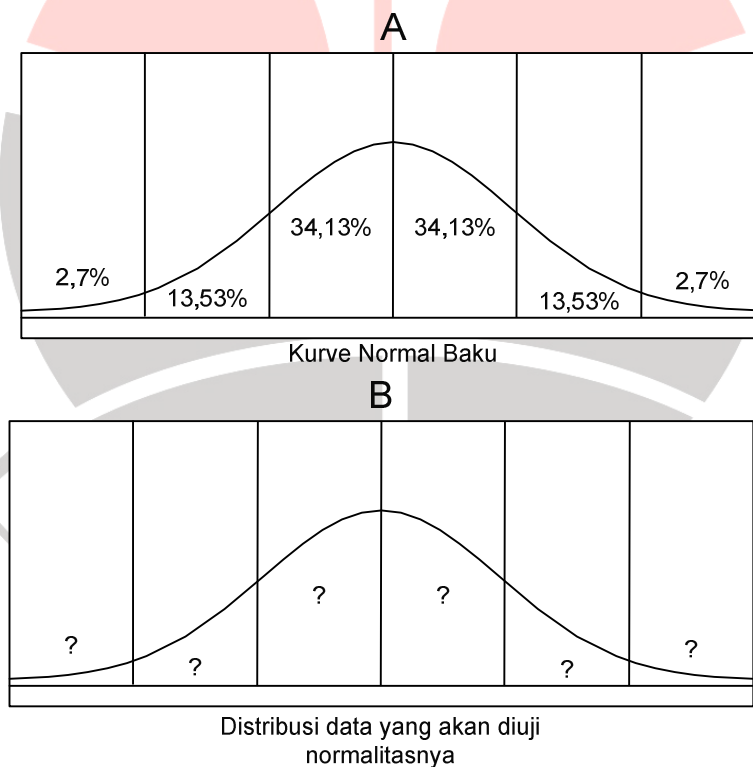
Gambar 3.3 Kurva Normal Baku
