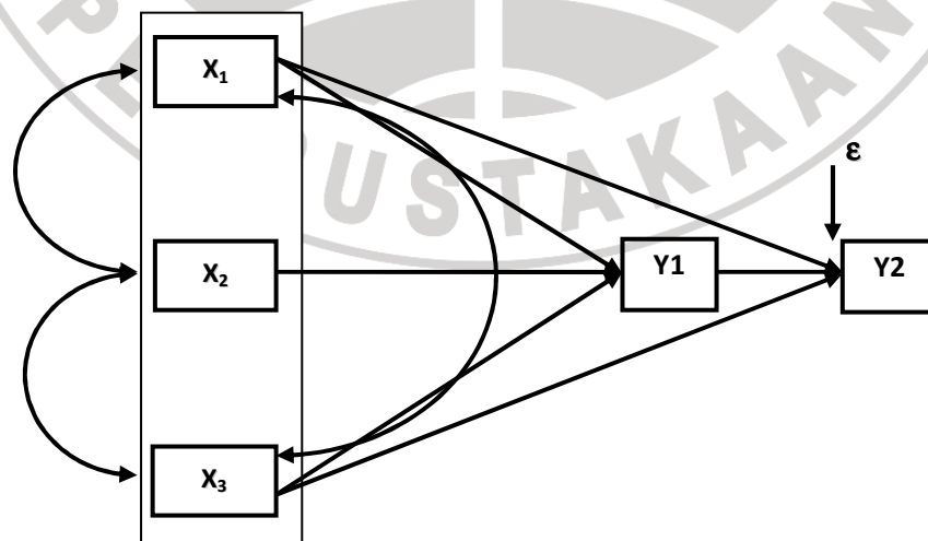
Gambar 3.7 Diagram Jalur Hipotesis 5
