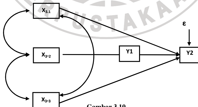
Gambar 3.10 Diagram Jalur Hipotesis 8
