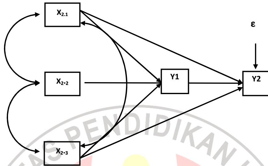
Gambar 3.9 Diagram Jalur Hipotesis 7
