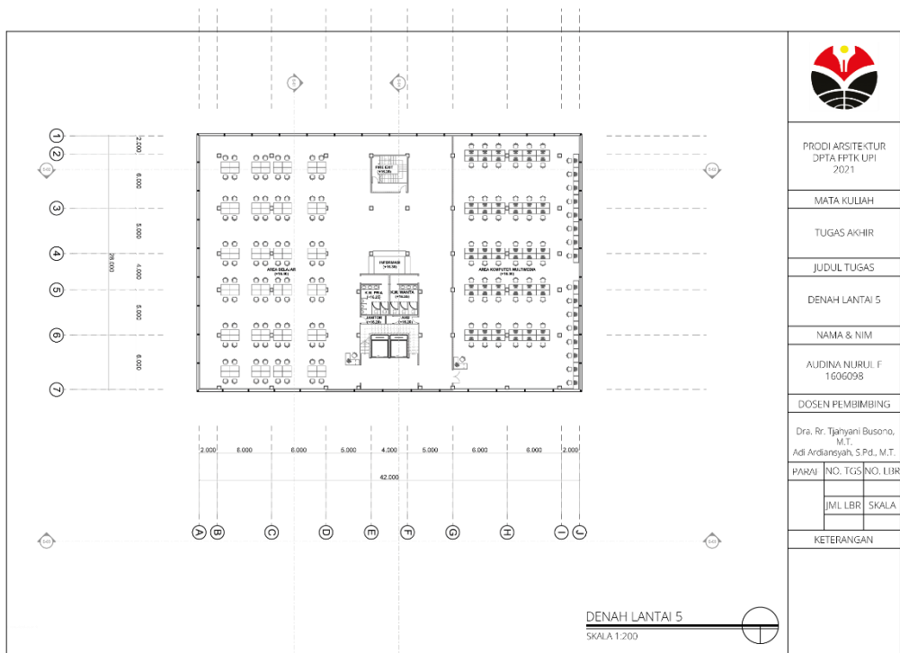
Gambar 5. 8 Denah Lantai 5
