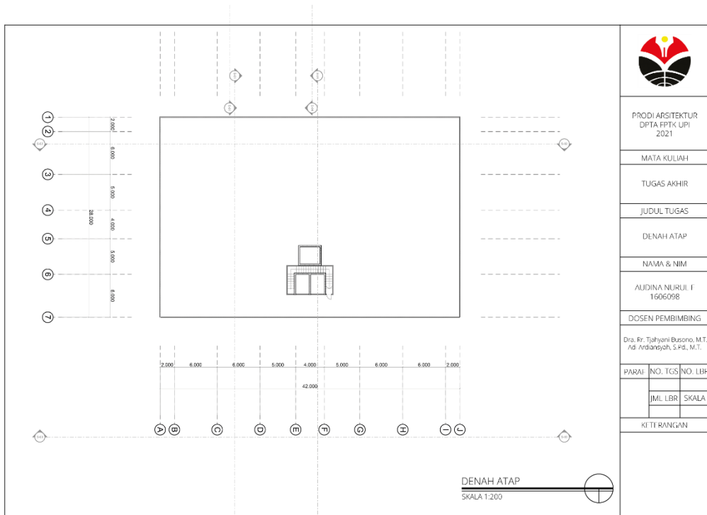
Gambar 5. 9 Denah Atap
