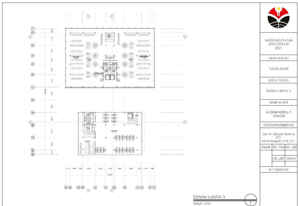
Gambar 5. 6 Denah Lantai 3
