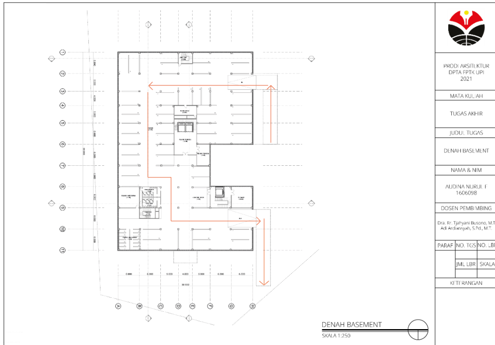
Gambar 5. 3 Denah Basement
