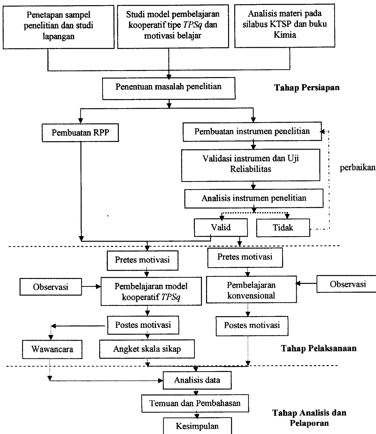
Gambar 3.1 Alur Penelitian
