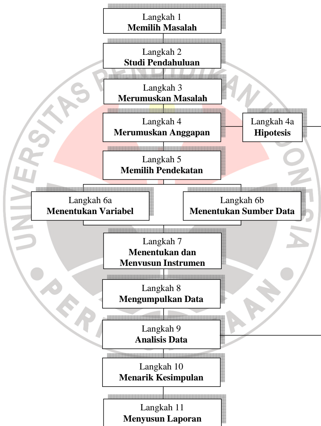
Gambar 3.6 Alur Penelitian
