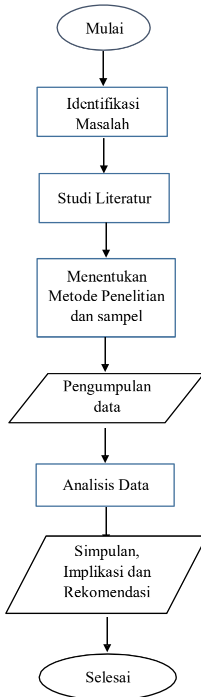
Gambar 3.2 Flowchart Penelitian
