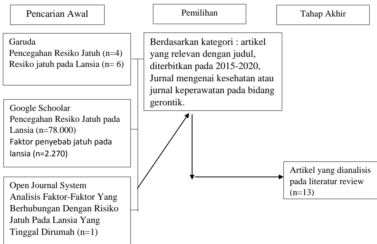
Gambar 3.3.1 Diagram PRISMA
