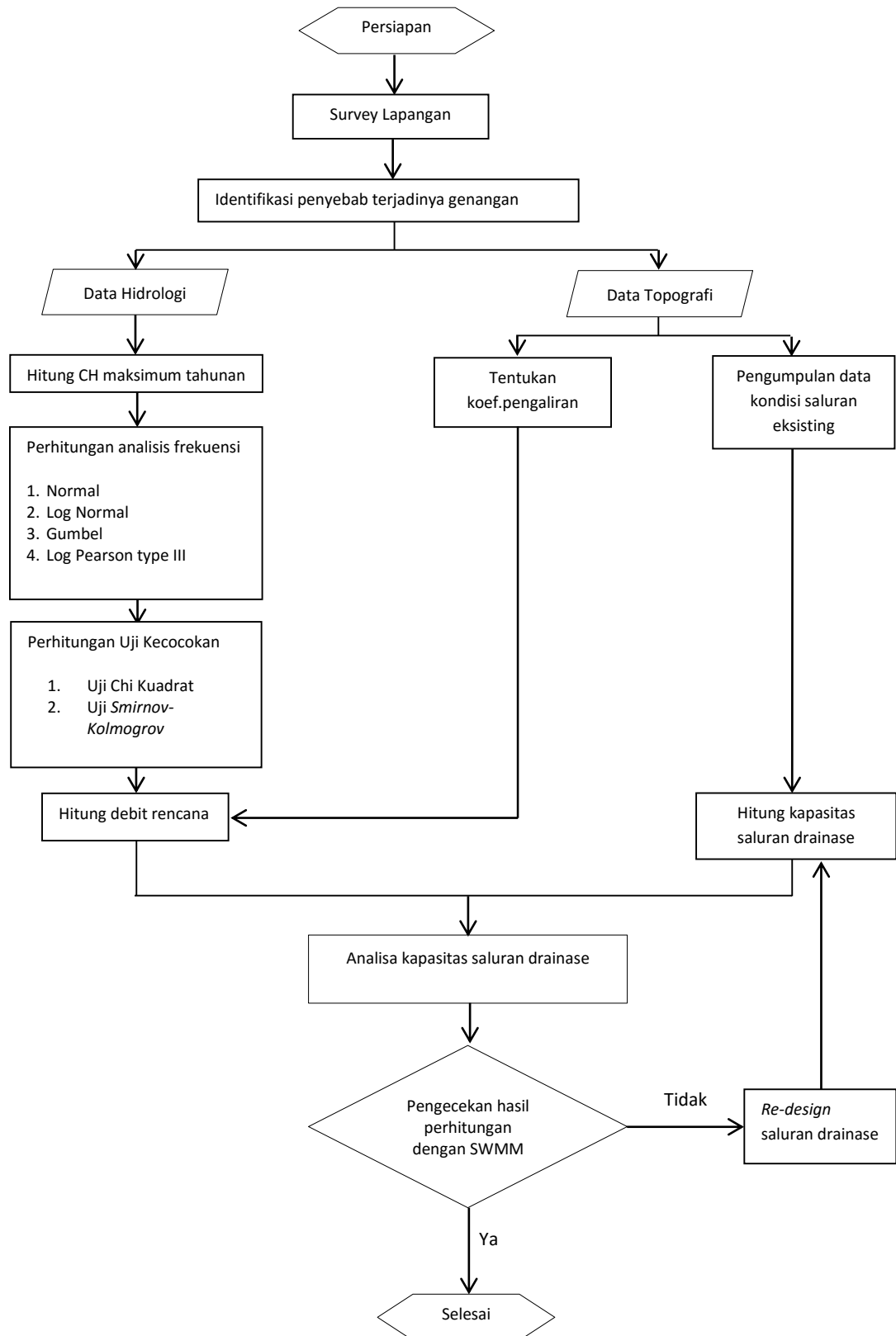
Gambar. 3.2.Bagan alur penelitian
