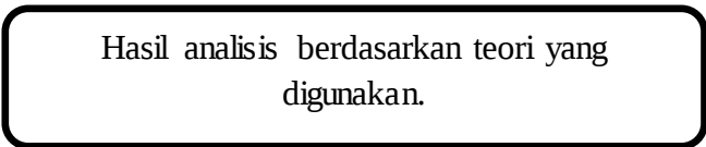
Diagram 3.1 Desain Penelitian
