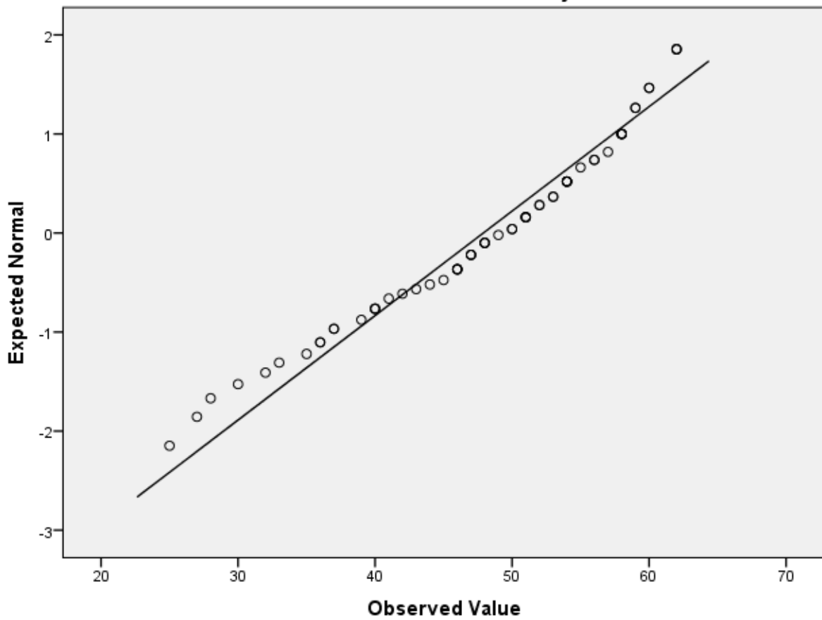
Normal Q-Q Plot of motivasi belajar
