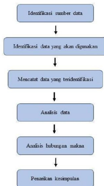
Gambar 3. 1 Metode Penelitian
