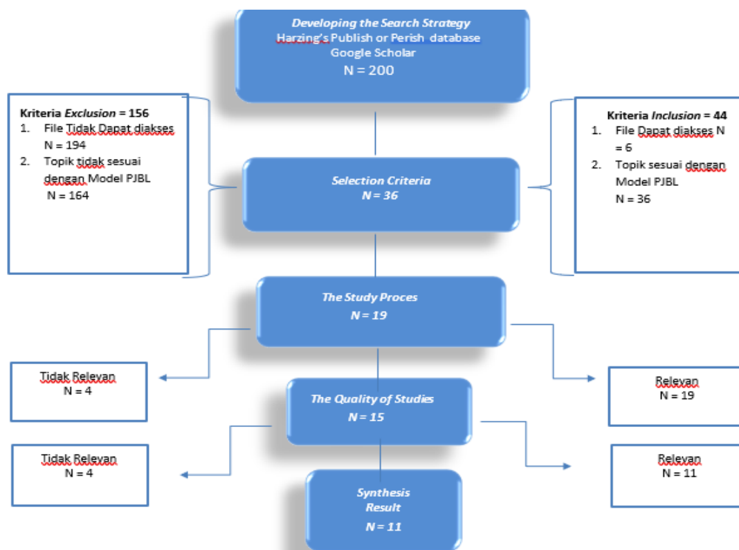
Gambar 1. Flowchart
