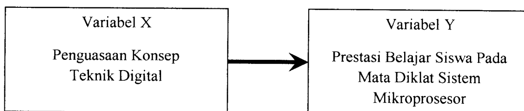
Gambar 3.1. Paradigma Penelitian
