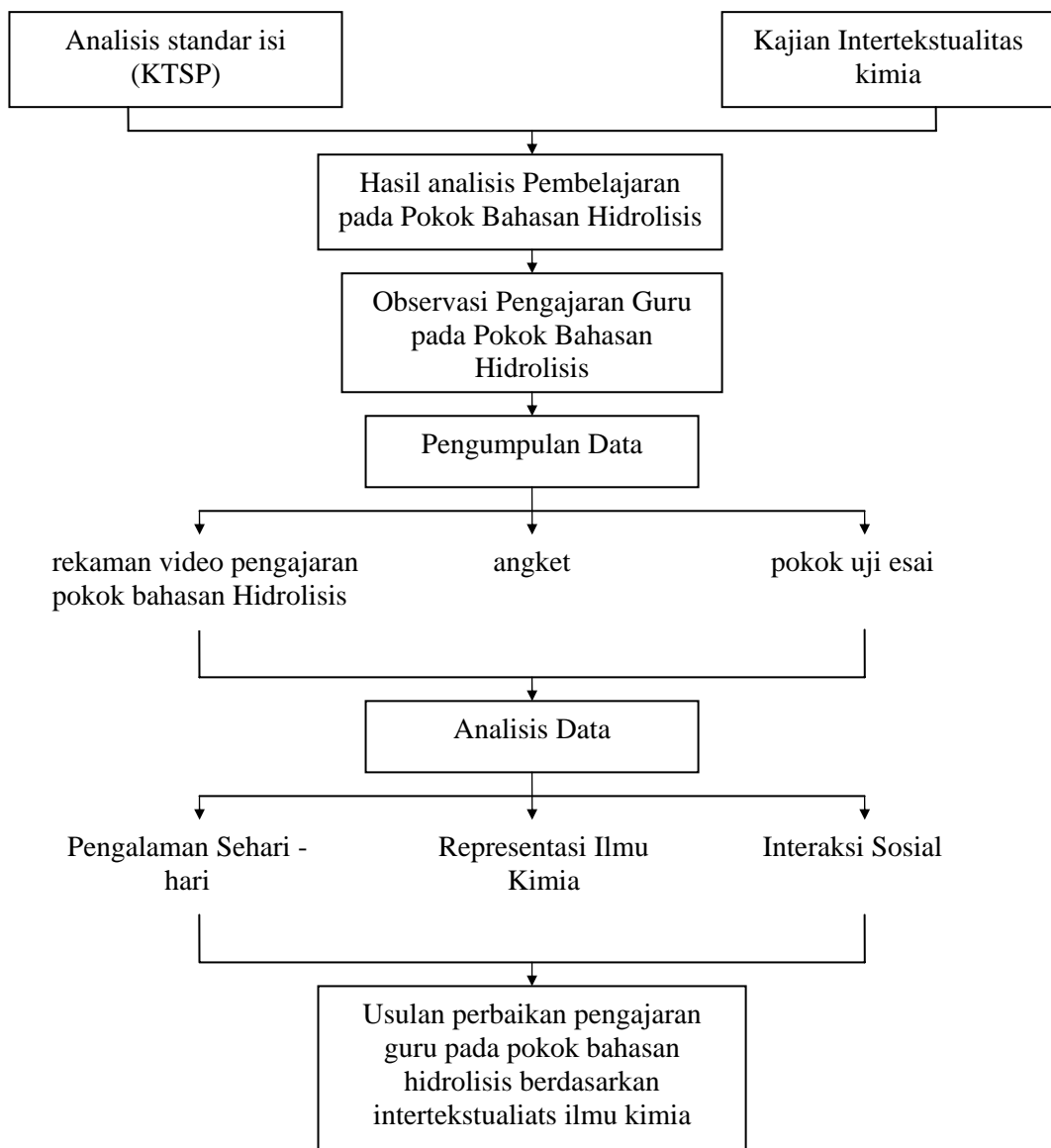
Gambar 3.1 . Diagram penelitian
